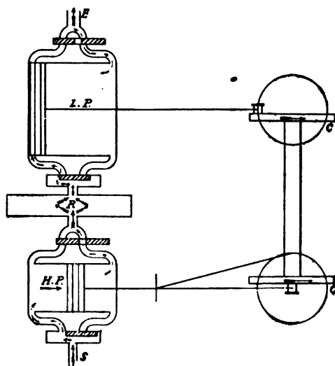
FIG. 242.—Diagram of a "Cross Compound" Steam Engine. The cranks, C and C', are at 90°. The high-pressure steam port is at S; the H. P. exhaust to L. P. cylinder at R, and the exhaust to atmosphere from the low-pressure cylinder, at E.
